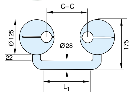
C-C 150 L 1 = 110 C-C 450 L 1 = 310
